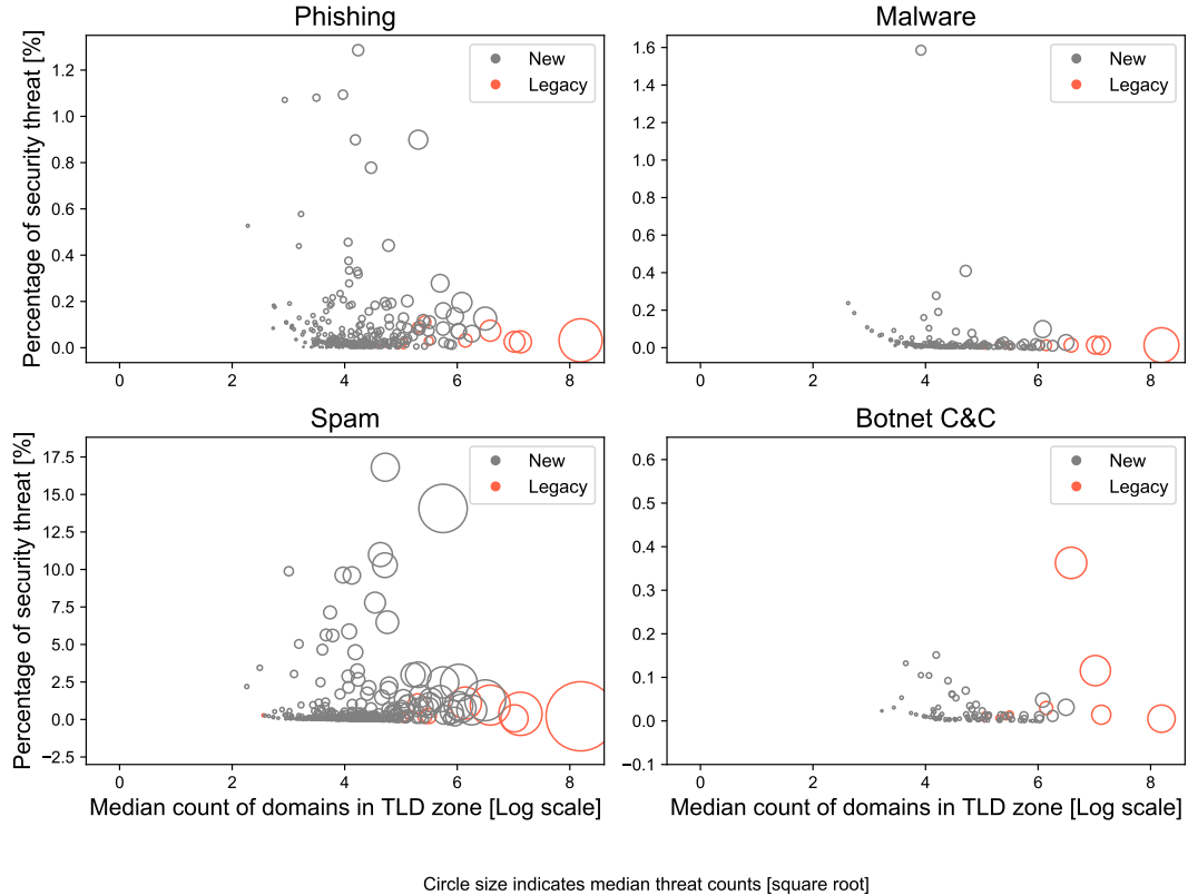
Figure 7: Percentage of domain names identified as security threats vs. counts of domains in TLD zones across different threat types
